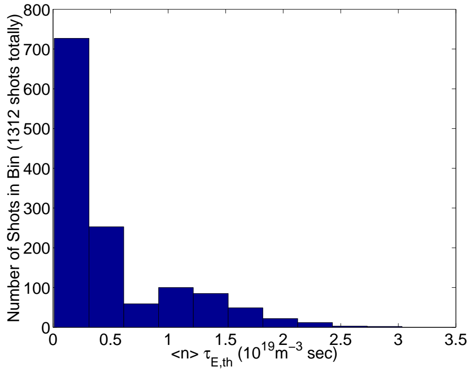
Fusion Confinement Parameter \langle n \rangle \tau_{E,th} from ITERL Database
