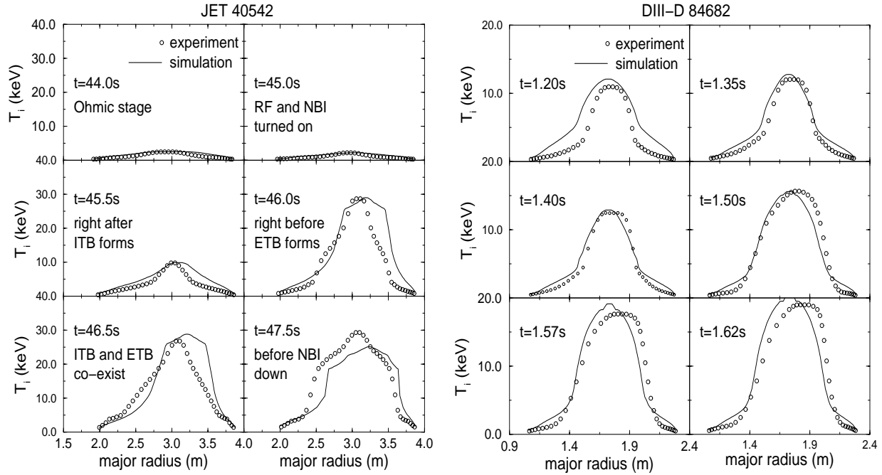
Figure 1: Experimental ion temperature profiles as a function of major radius (open circles) and the corresponding optimized simulation profiles with Hahm-Burrell flow shear stabilization (solid curves) at six time slices for JET shot 40542, and DIII-D shot 84682.
